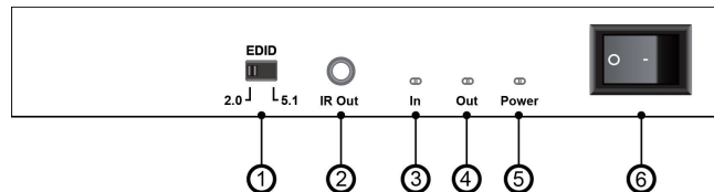
Front Panel
